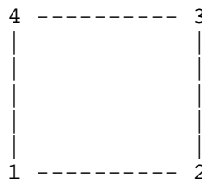
ESMC_MESHELEMENTTYPE_QUAD
