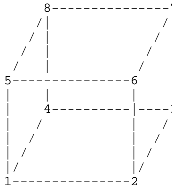
ESMC_MESHELEMENTTYPE_HEX
