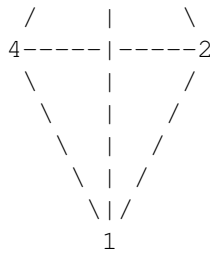
ESMF_MESHELEMENTTYPE_TETRA
