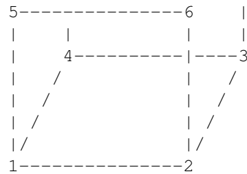
ESMF_MESHELEMENTTYPE_HEX
