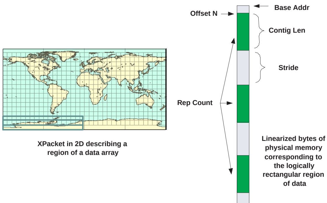
Figure 21: How an Exchange Packet (XPacket) describes the memory layout for a rectangular hypercube of data.
