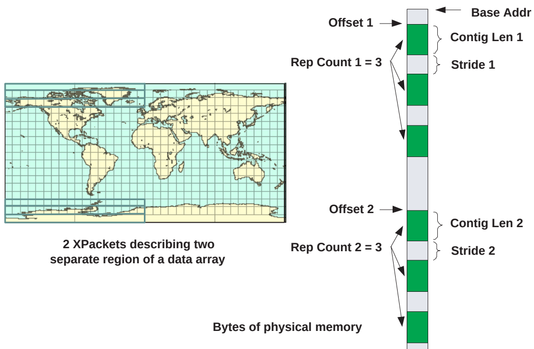
Figure 23: When there are multiple XPackets destined for the same remote PET there are more options for how to order the contiguous pieces into a packed buffer.
